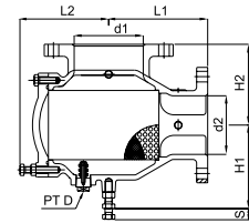
FLANGED TYPE
