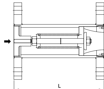
YFC-1F
