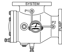
FLANGED TYPE(STANDARD)
