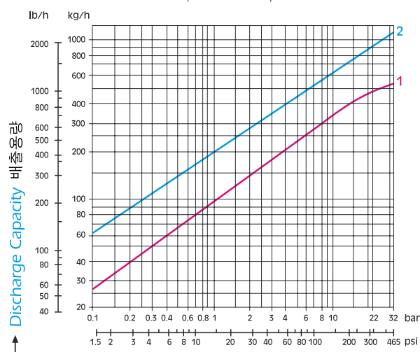
Discharge Capacities 배출용량 ( 3/8" - 3/4" )
