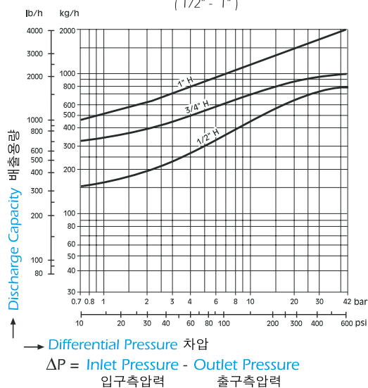
Discharge Capacities 배출용량 (1/2" - 1")
