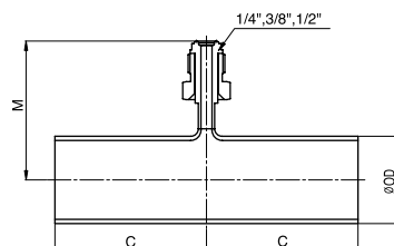
MALE TYPE
