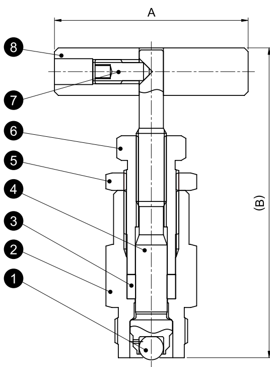
Large Bonnet Valve
