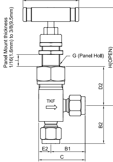
Angle Pattern
