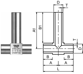
MICRO EXTENDED BRANCH LEG TEE
