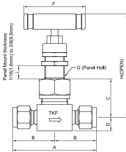
Straight Pattern
