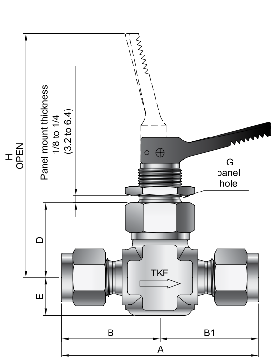
Straight Pattern
