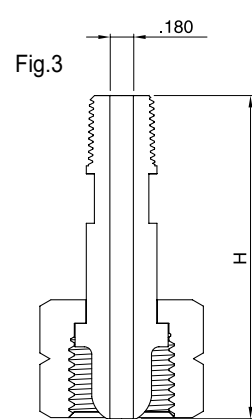
NPT MALE
