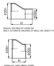
Manual-Welding of Large Dia. Side×Automatic Welding of Small Dia. Sides & Manual-Welding Type Eccentric Reducer [REB] (125A~300A)
