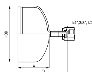
FEMALE TYPE
