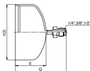
MALE TYPE
