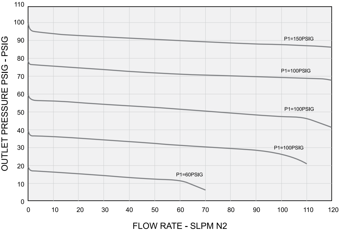
DISCHARGE CHARACTERISTICS CURVE
