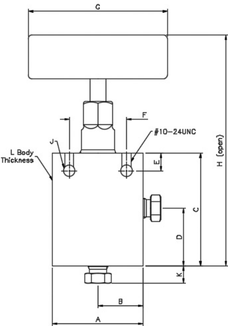
2-WAY ANGLE
