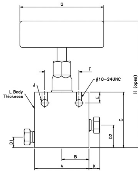
2-WAY STRAIGHT
