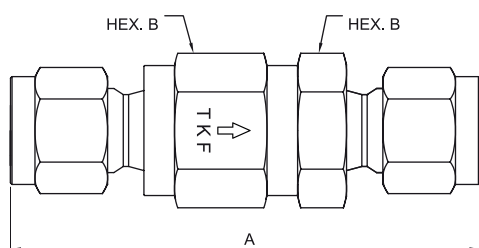
ICH1 SERIES
