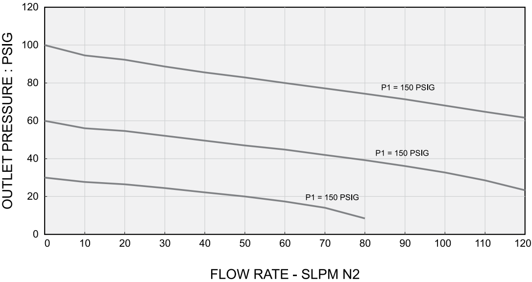
DISCHARGE CHARACTERISTICS CURVES
