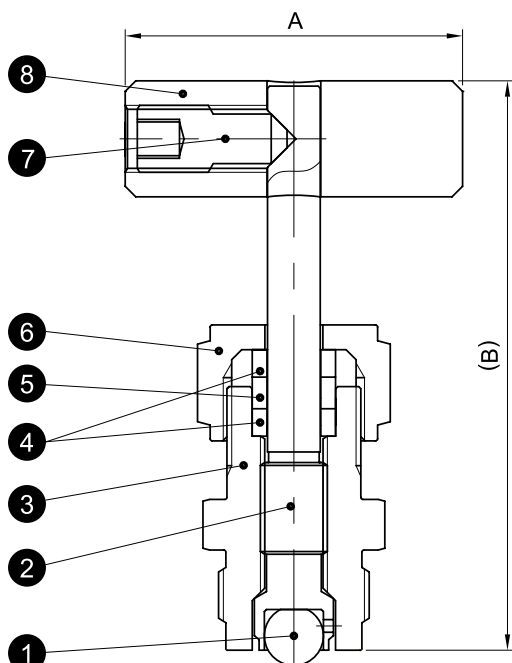
Small Bonnet Valve
