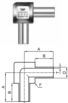
90° ELBOW
