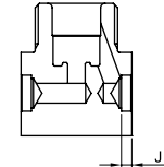
Socket weld end connection
