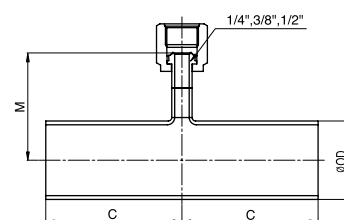
FEMALE TYPE
