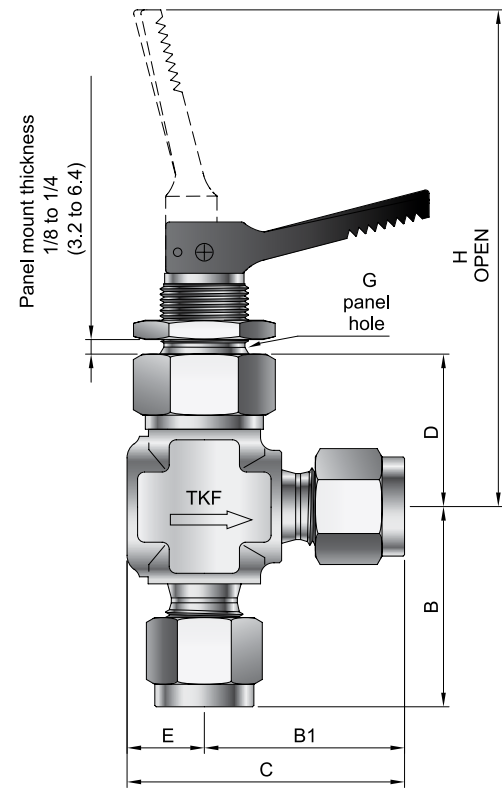
Angle Pattern
