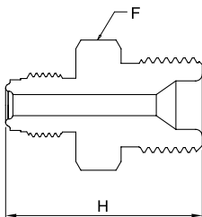
FACESEAL MALE
