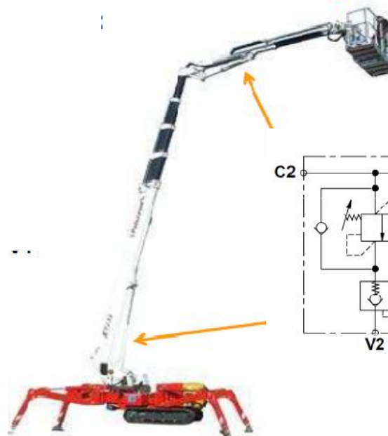
Counterbalance Valves With Double Safety
