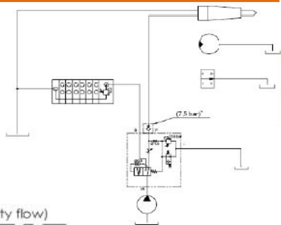
HAMMER VALVES
