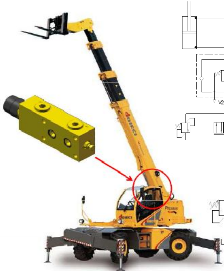
BOOM LIFTING
