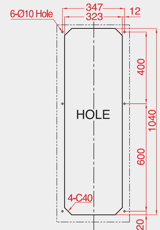
MOUNTING CUT-OUT
