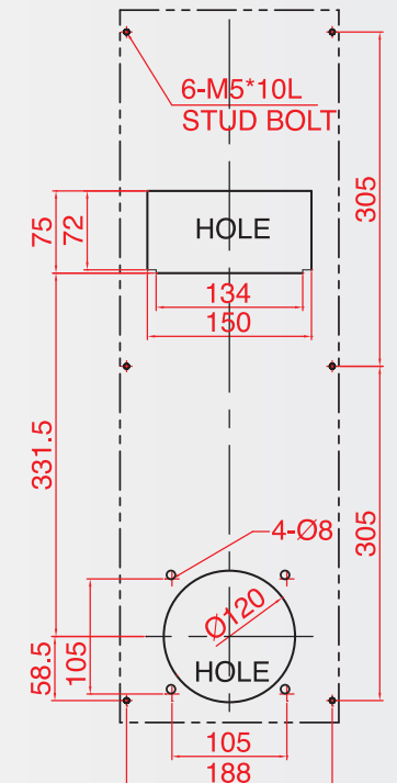
MOUNTING CUT-OUT
