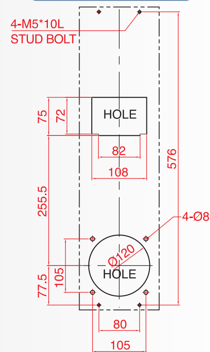
MOUNTING CUT-OUT
