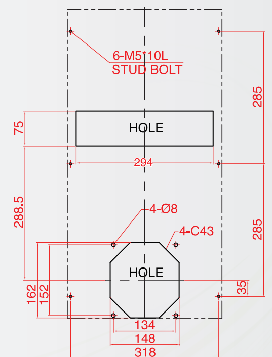
MOUNTING CUT-OUT
