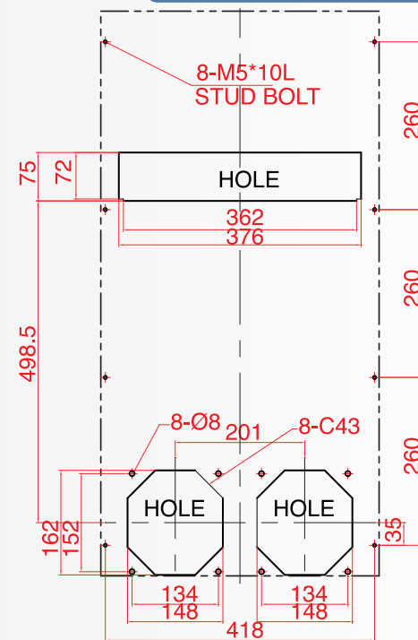
MOUNTING CUT-OUT
