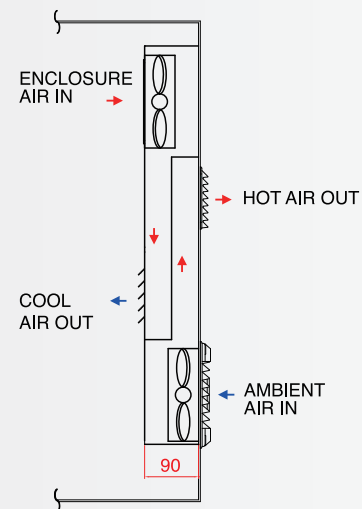
Switch Cabinet
