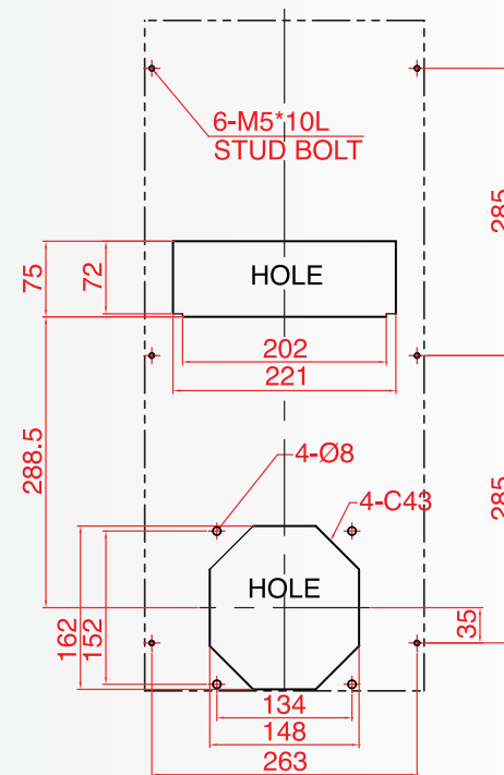
MOUNTING CUT-OUT
