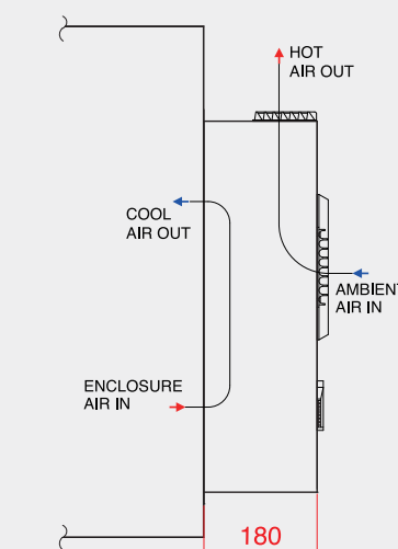
Switch Cabinet
