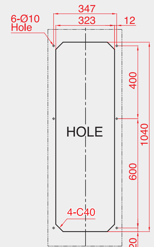
MOUNTING CUT-OUT
