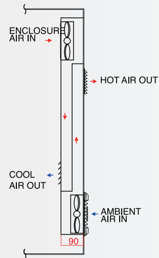
Switch Cabinet
