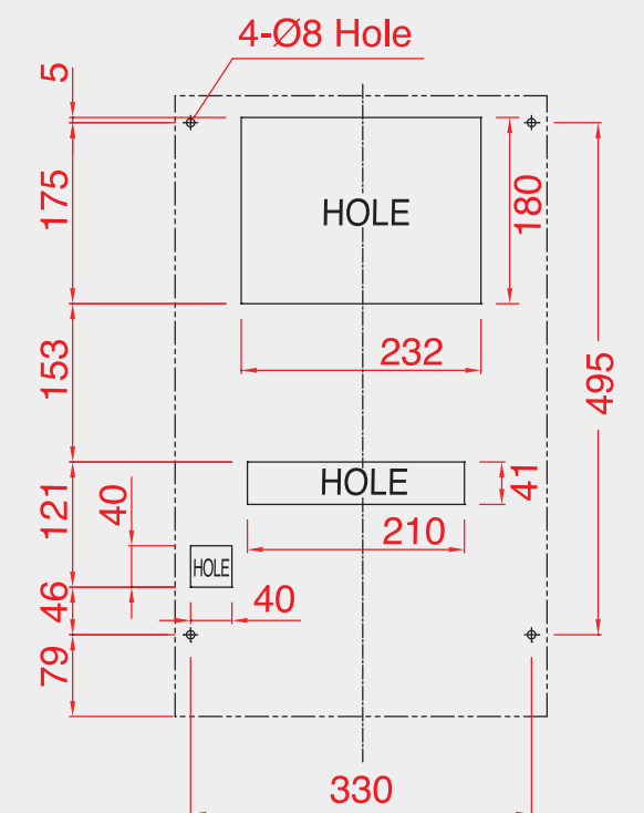
MOUNTING CUT-OUT
