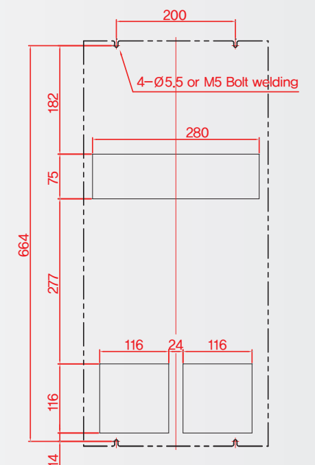
MOUNTING CUT-OUT
