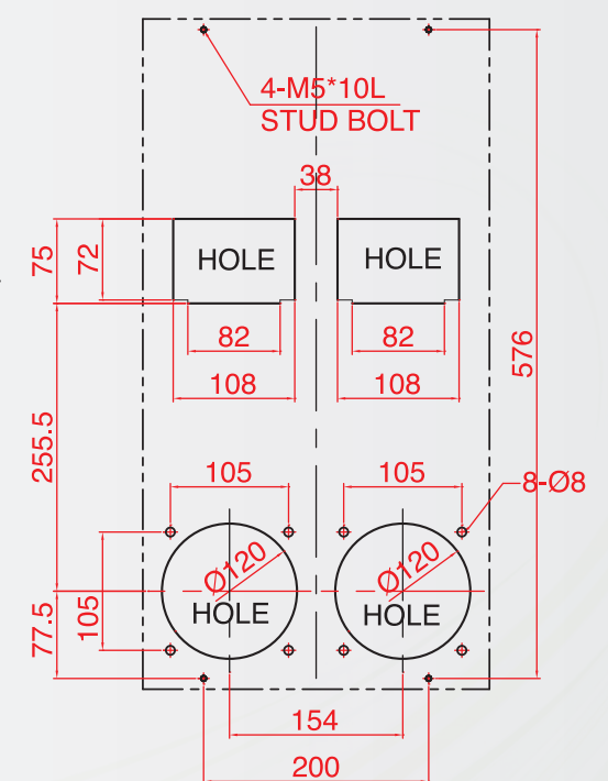
MOUNTING CUT-OUT
