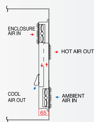
Switch Cabinet
