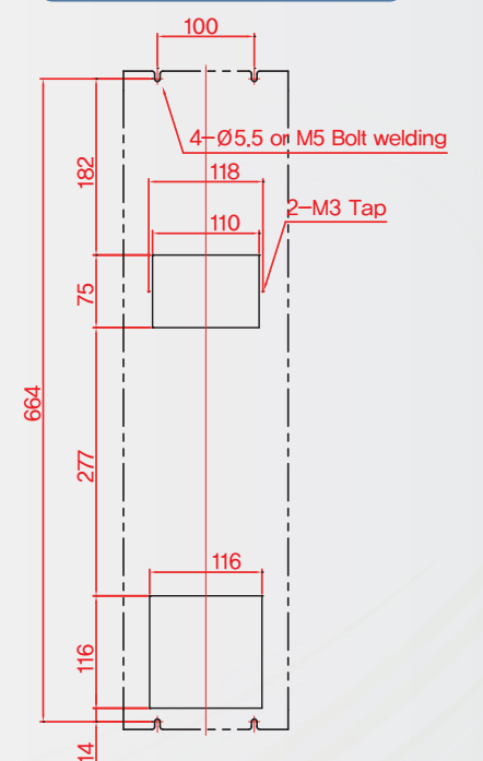
MOUNTING CUT-OUT
