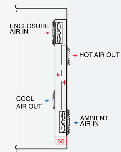
Switch Cabinet
