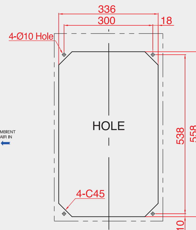
MOUNTING CUT-OUT
