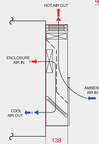
Switch Cabinet
