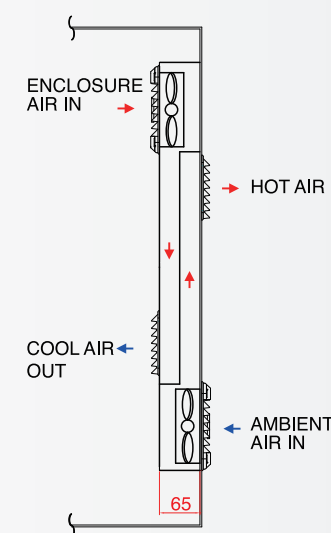
Switch Cabinet
