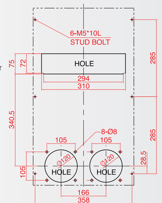
MOUNTING CUT-OUT
