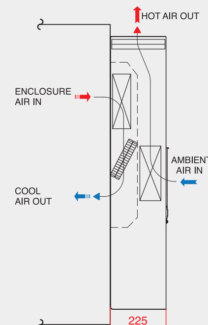
Switch Cabinet
