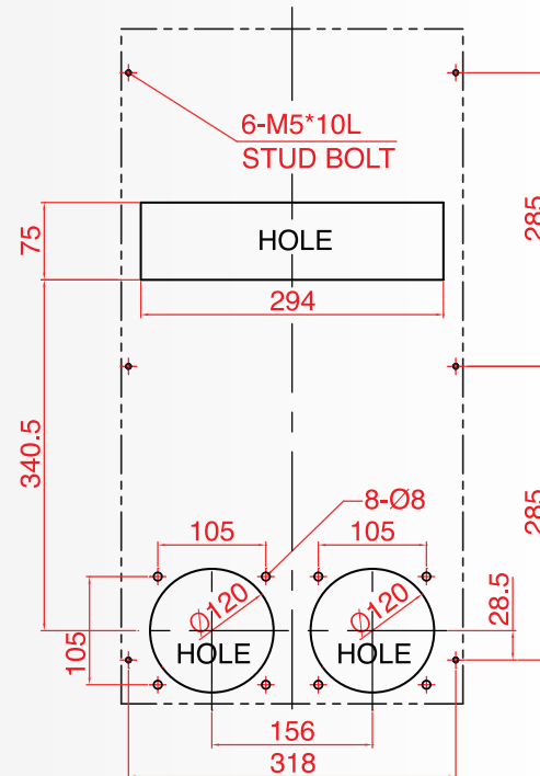
MOUNTING CUT-OUT
