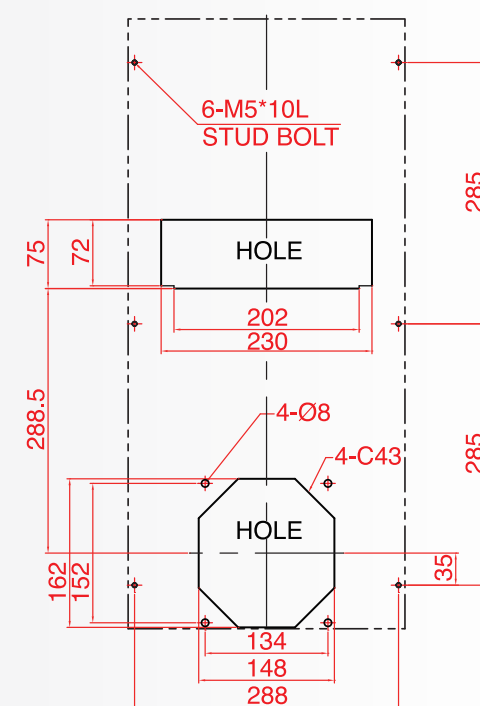
MOUNTING CUT-OUT
