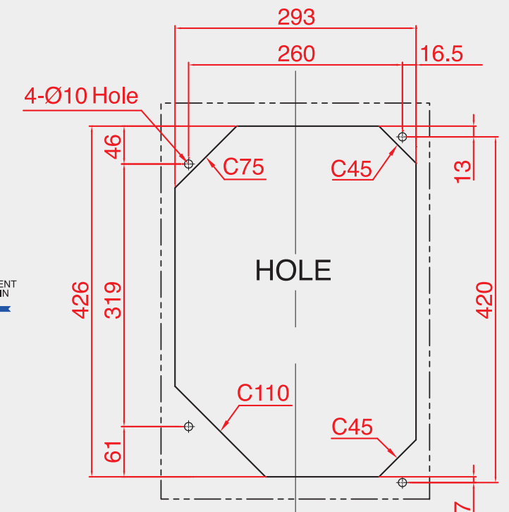
MOUNTING CUT-OUT
