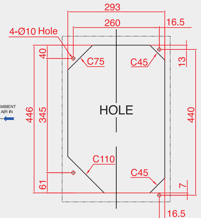
MOUNTING CUT-OUT
