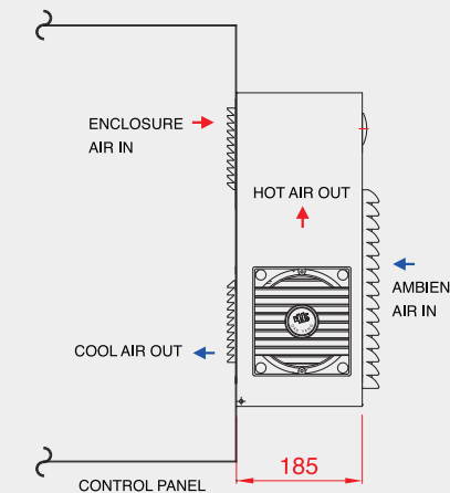
Switch Cabinet
