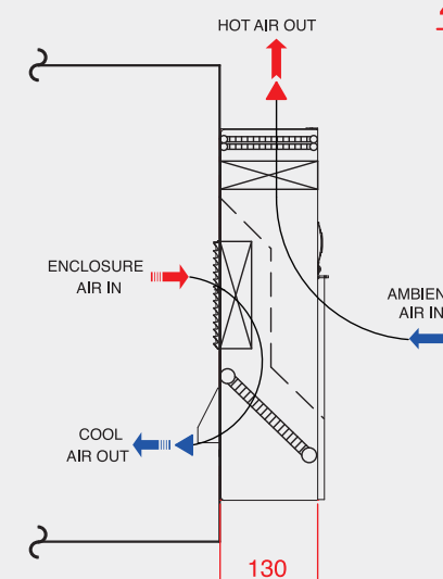
Switch Cabinet
