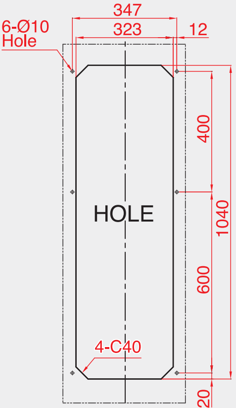
MOUNTING CUT-OUT
