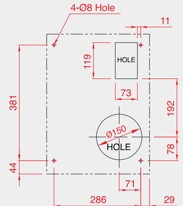
MOUNTING CUT-OUT
