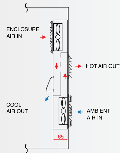
Switch Cabinet
