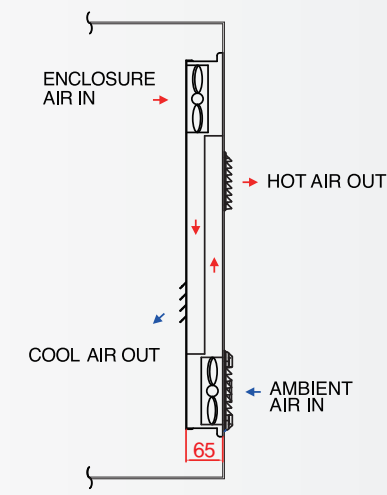
Switch Cabinet
