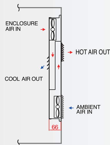
Switch Cabinet
