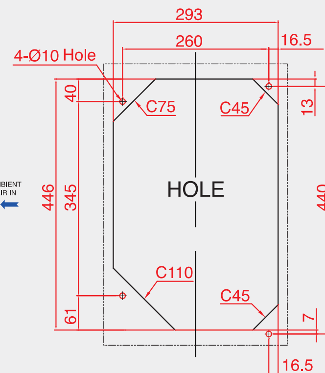
MOUNTING CUT-OUT
