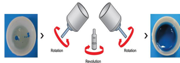
Centrifugal rotation of paste mixer/inter mixer.
