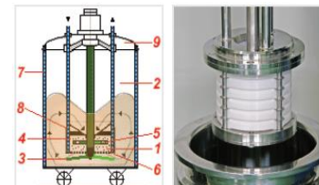
Basket mill
