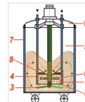
Basket mill
