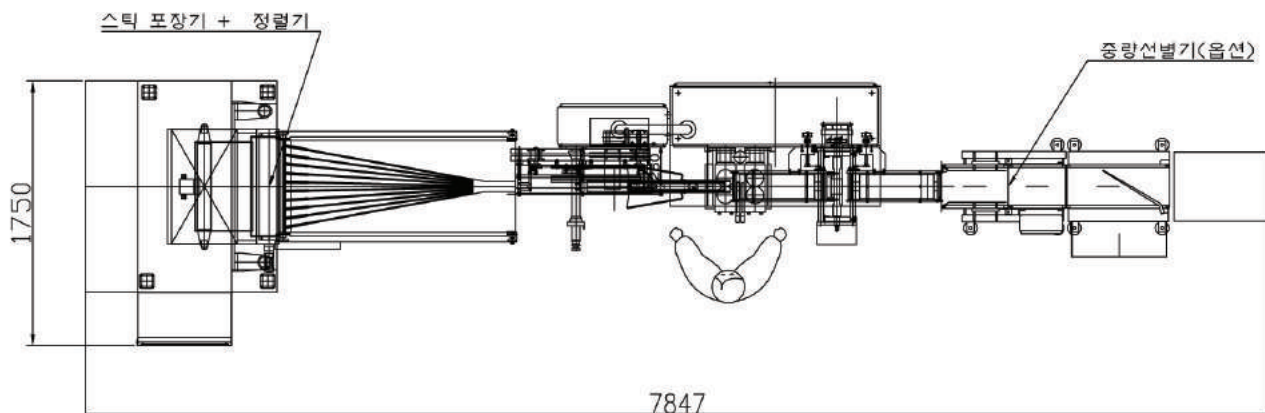
Stick & Pillow Layout
