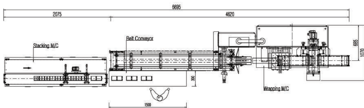
Tea Packaging Line Layout
