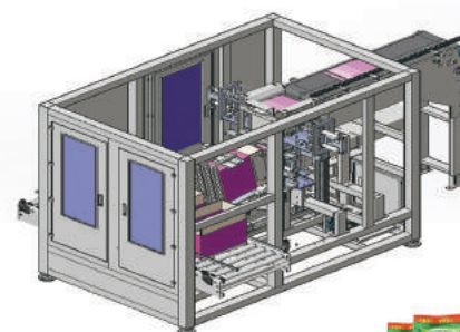
Flat Bags drop into carton
