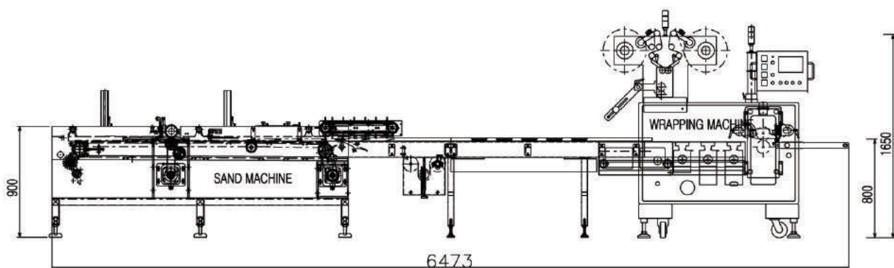
Sand Line Layout
