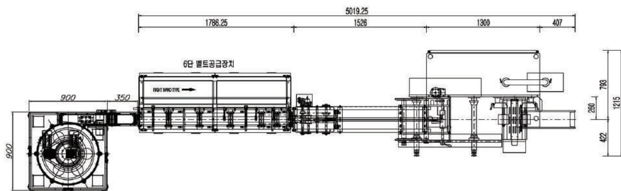
Rotary Feeder Layout
