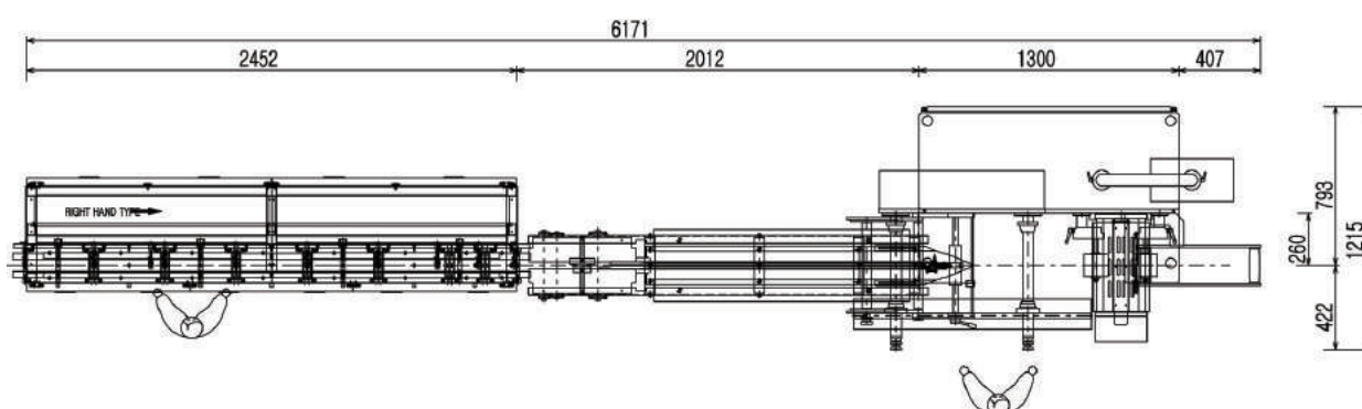
Auto Feeder Line Layout
