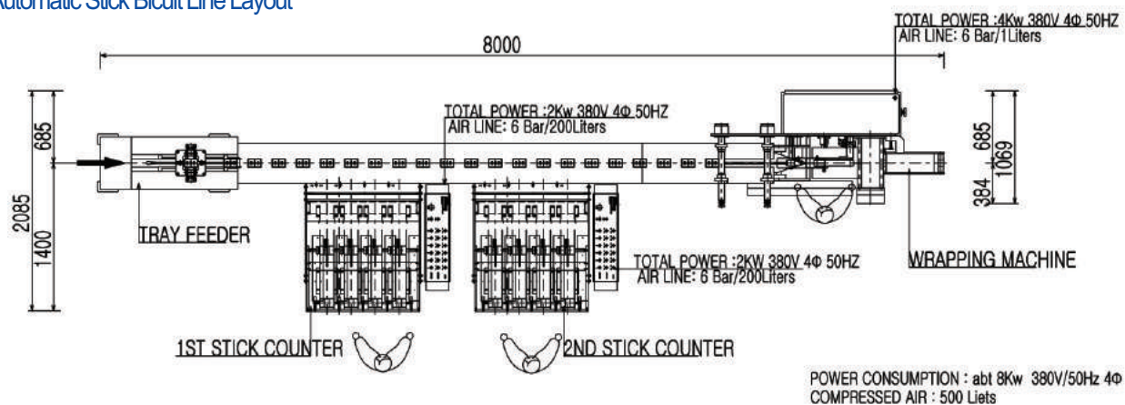
Full Automatic Stick Biscuit Line Layout
