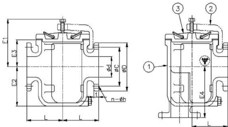
SERIES F 7203 - S type Mud Box
