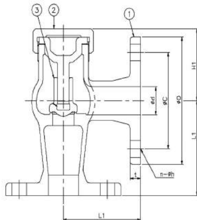
SERIES F 7416 Lift Check Angle Valve
