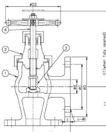
SERIES F 7412 Angle Valve
