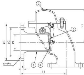
SERIES F 3058 Angle Storm Valve
