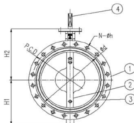
Flange Type
