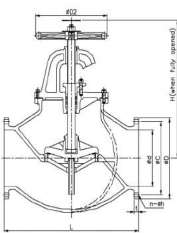
SERIES F 7311 Globe Valve
