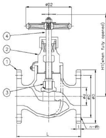
SERIES F 7409 Globe Check Valve
