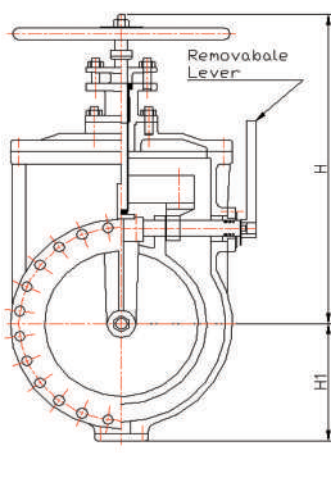
SERIES HSN SCIG 01 Inert Gas Line Valve
