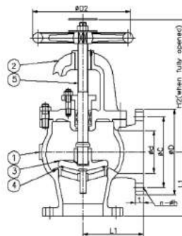
SERIES F 7376 Angle Check Valve
