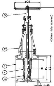
SERIES F 7360 (Size 450A~500A) Gate Valve
