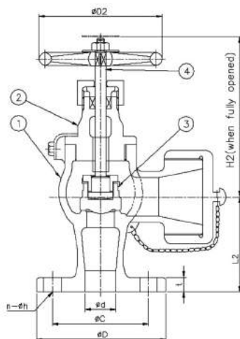
SERIES F 7334 - Hose Angle Valve
