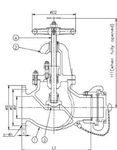
SERIES F 7334 - Hose Globe Valve
