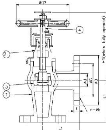
SERIES F 7404 Hull Angle Valve
