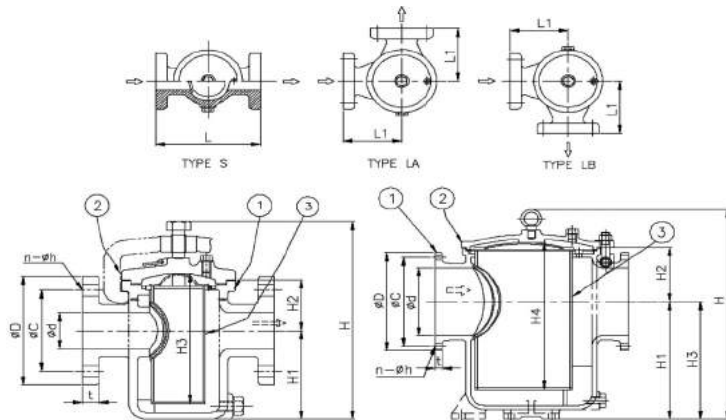
SERIES F 7121 [25A~100A] Water Strainer
