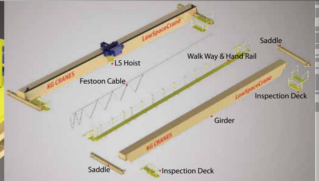
Disassembly Drawing
