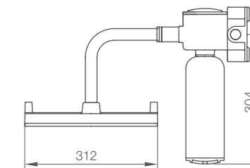
90° BRACKET TYPE
