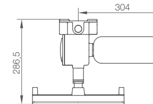
CEILING TYPE
