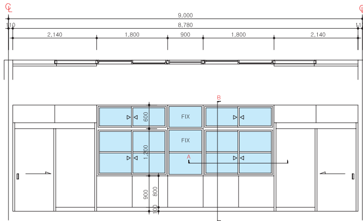
SLIDING WINDOW ELEV.
