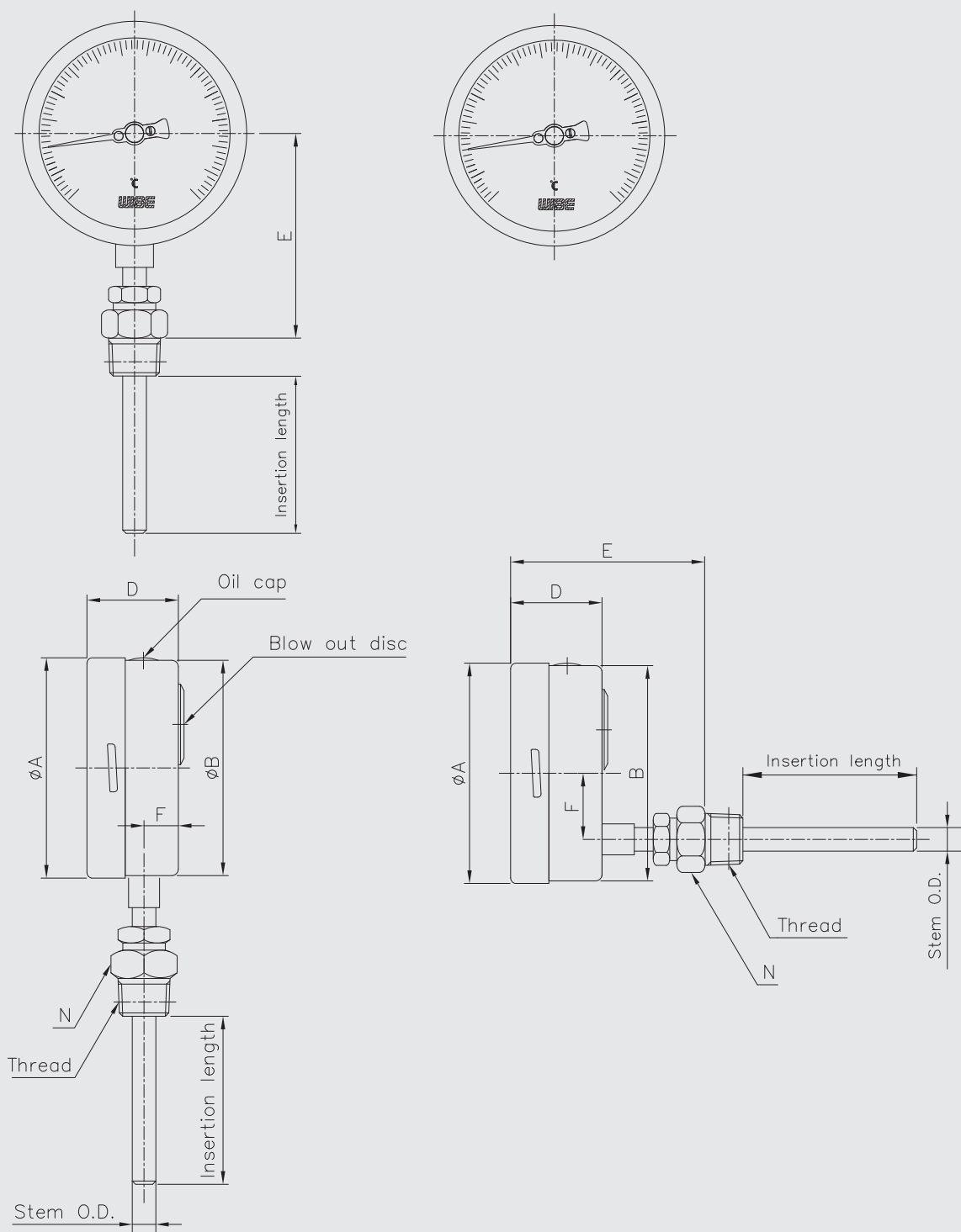
Dimensions (mm)
