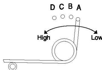
Detection Torque Adjustment Spring Setting
