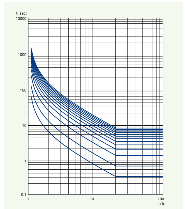
IEC-LI:Longtime Inverse Time
