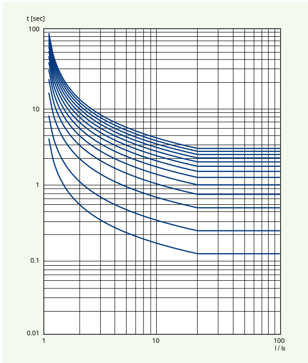
IEC-SI:Standard Inverse Time
