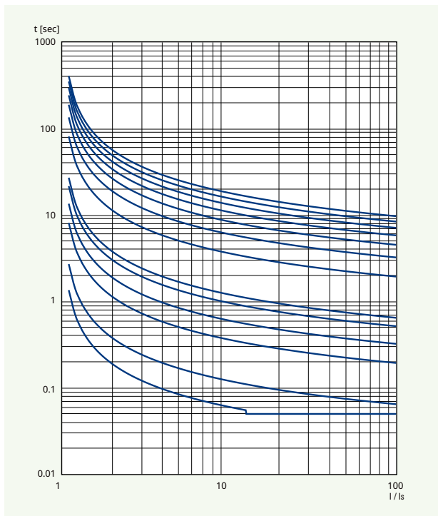
IEEE-MI : Moderately Inverse Time)
