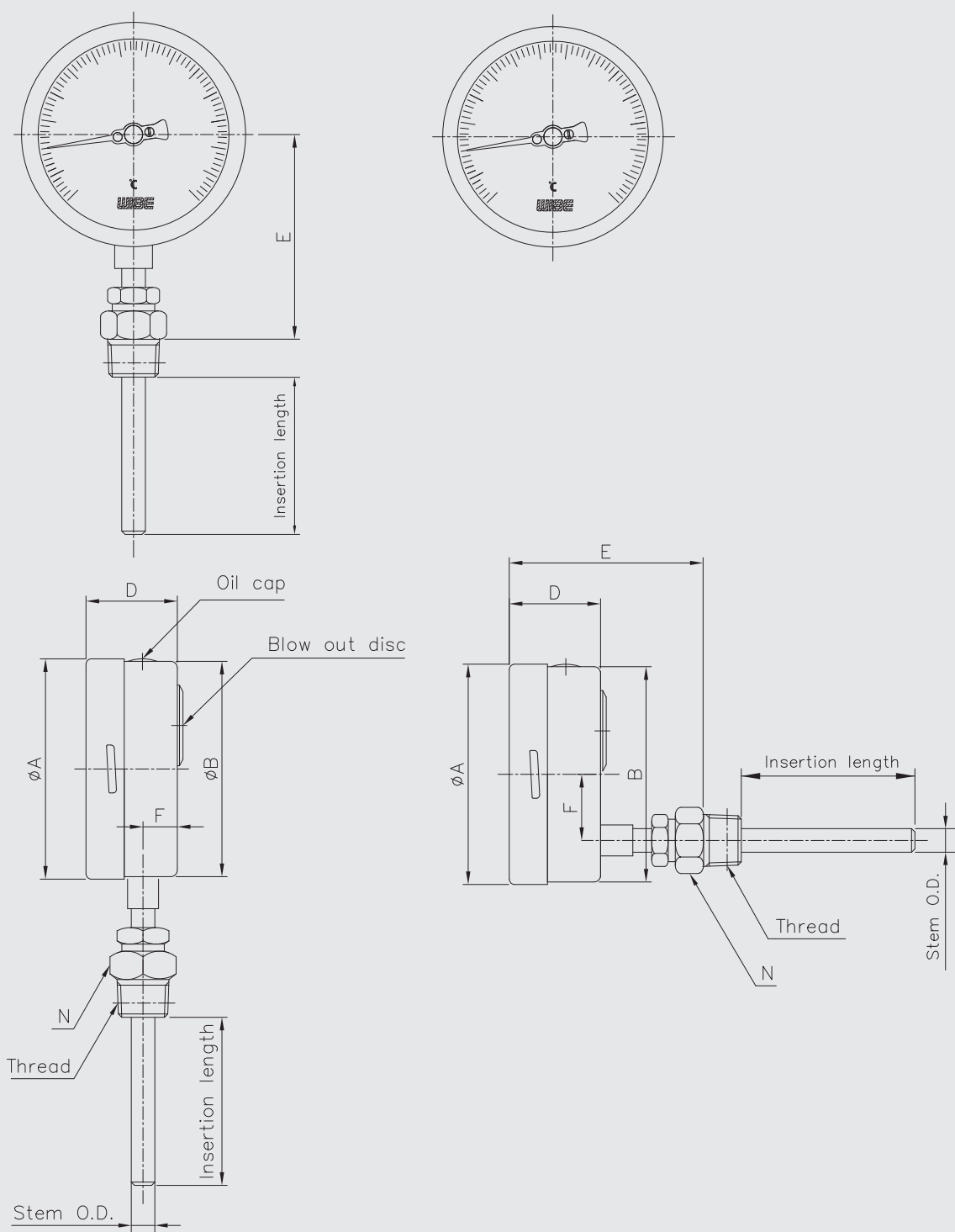
Dimensions (mm)
