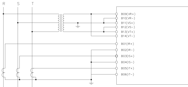
(4) 3P 3W: 3CT, 2PT
