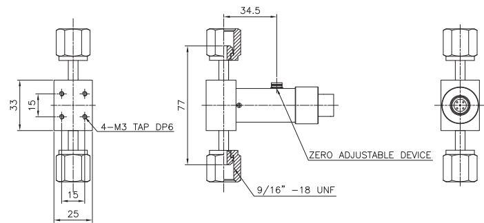
FLOW THROUGH FEMALE
