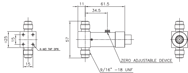
FLOW THROUGH MALE
