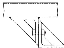
Supporting brackets
