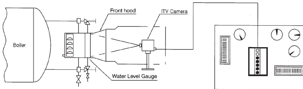
Television Observation Device
