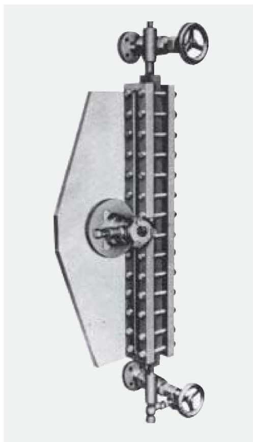
Illuminator Explosion-Proof JIS · d2G4
