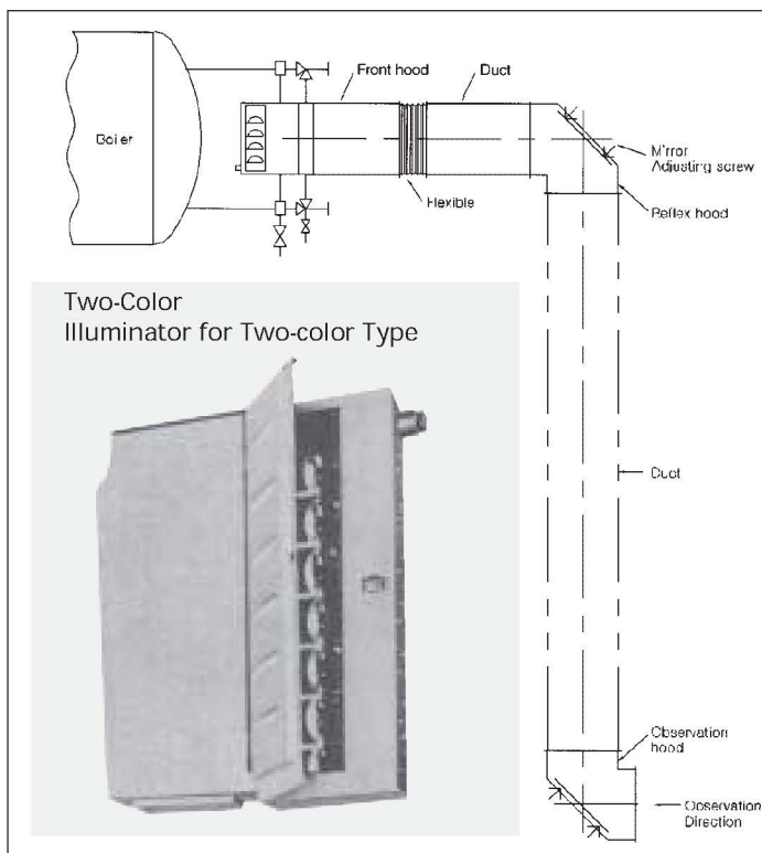
Reflex Mirror Hood and Observation Mirror Hood
