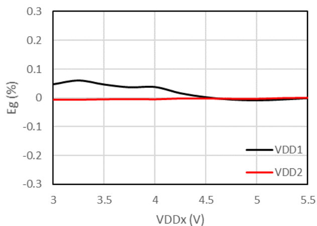
Figure 7-2 Gain Error vs Supply Voltage
