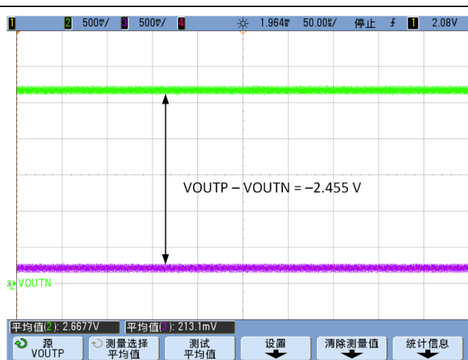
Figure 9-5 Typical Negative Clipping Output Waveform
