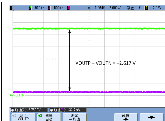
Figure 9-4 Typical Fail-safe Output Waveform
