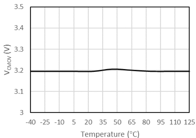
Figure 7-5 High-Side V_{CMOV} vs Temperature
