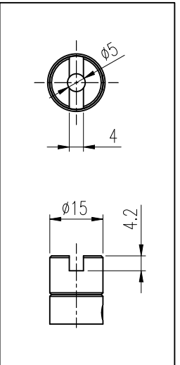
L/S Connection
