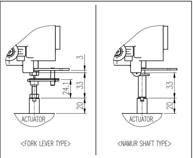
FEEDBACK LEVER
