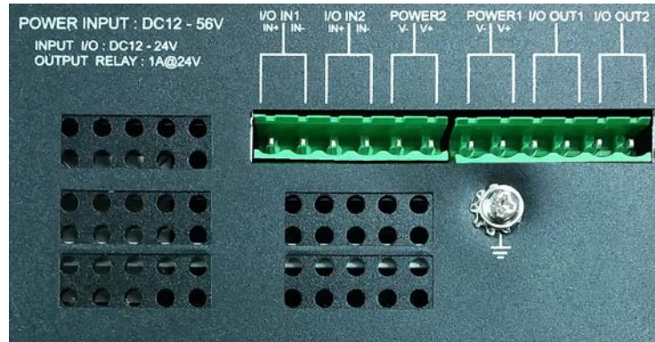
Rear Panels of SFC8000HP
