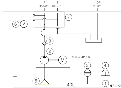
HYD. CIRCUIT DIAGRAM
