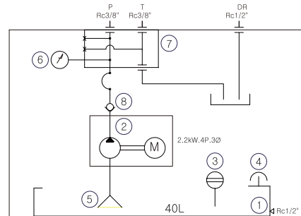
HYD¹ CIRCUIT DIAGRAM
