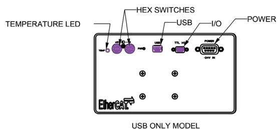
VS70-MC back panels for different models
