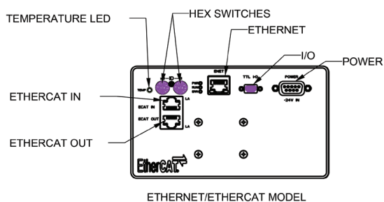
VS70-MC back panels for different models
