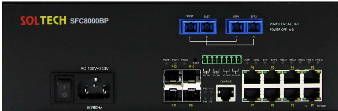
Rear Panels of SFC8000BP
