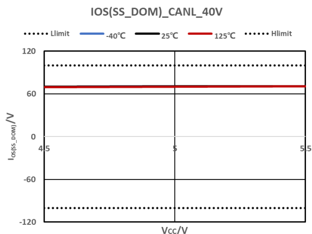
Figure 7-12 Driver Output Short-circuit Current
