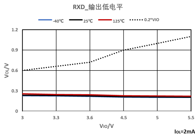
Figure 7-15 RXD Low-Level Output
