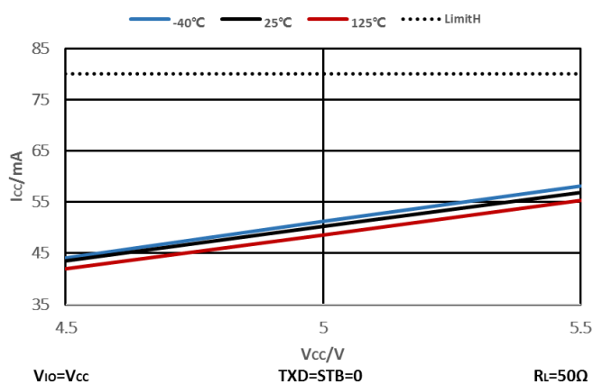
Figure 7-3 V_{CC} Supply Current @ Dominant ( R_L = 50\Omega )
