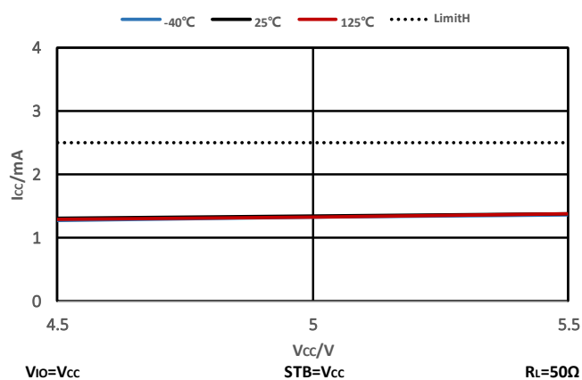
Figure 7-2 V_{CC} Supply Current @ Recessive
