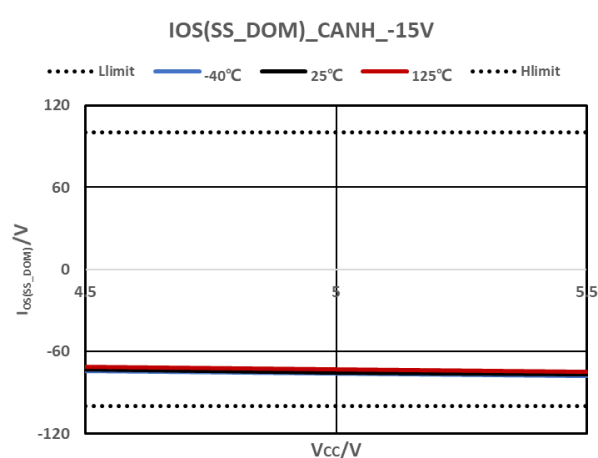
Figure 7-13 Driver Output Short-circuit Current
