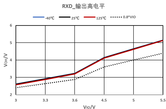
Figure 7-14 RXD High-Level Output
