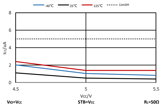
Figure 7-1 V_{CC} Supply Current @ Standby
