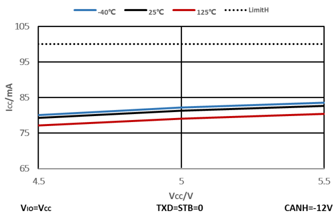
Figure 7-5 V_{CC} Supply Current @ Bus Fault
