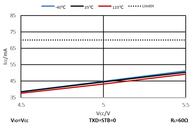
Figure 7-4 V_{CC} Supply Current @ Dominant ( R_L = 60\Omega )
