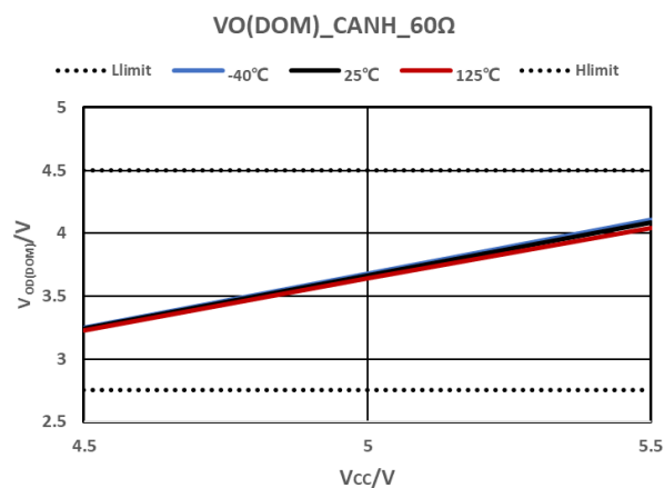
Figure 7-17 Differential Output Voltage ( R_L = 60\Omega )
