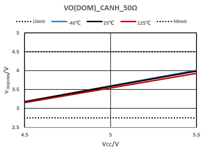
Figure 7-16 Differential Output Voltage ( R_L = 50\Omega )
