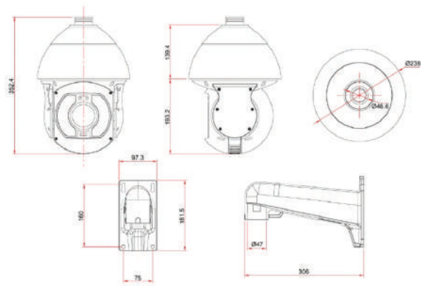
FW8709-FNR 2MP Laser and IR Speed Dome
