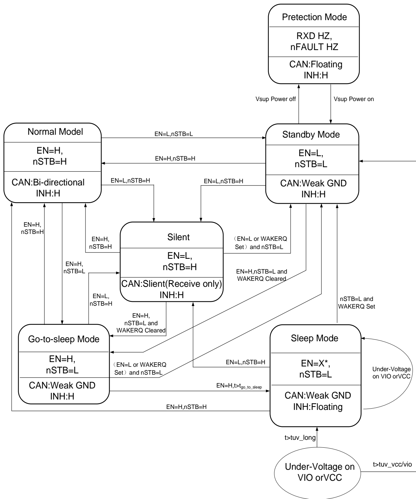
Figure 9-4. State Diagram
