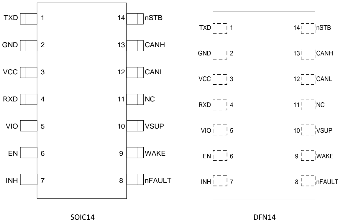
Figure 6-1. CA-IF1043 Pin Configuration
