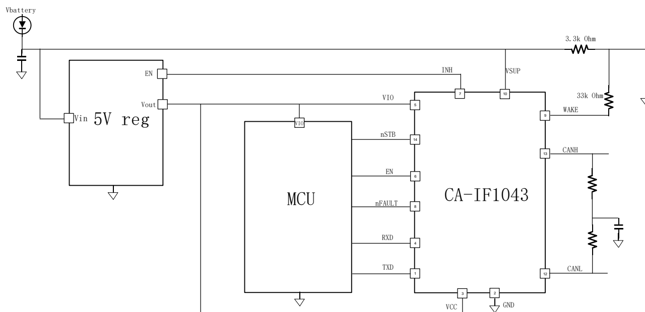
Figure 10-1. Typical Application Circuit for the CA-IF1043x with +5V supply
