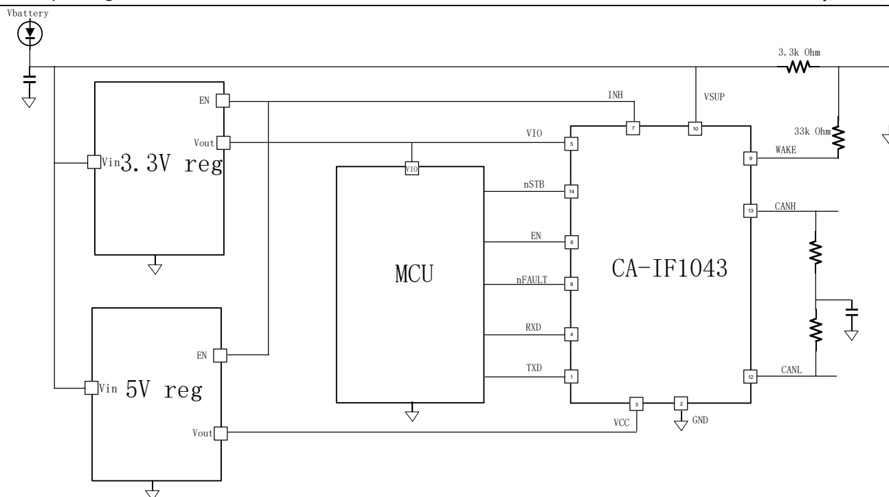
Figure 10-2. Typical Application Circuit for the CA-IF1043x with +3.3V supplies
