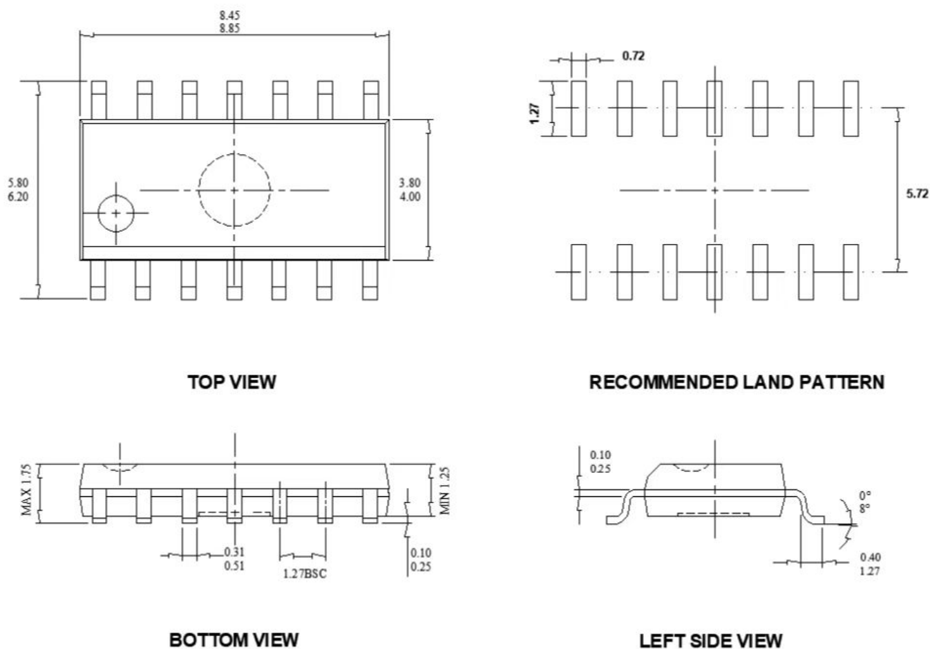
Figure 11-1. SOIC14 Package Outline
