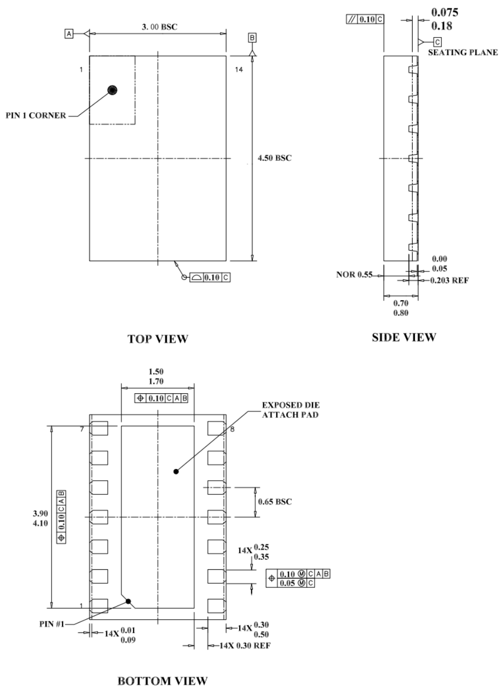
Figure 11-2. DFN14 Package Outline
