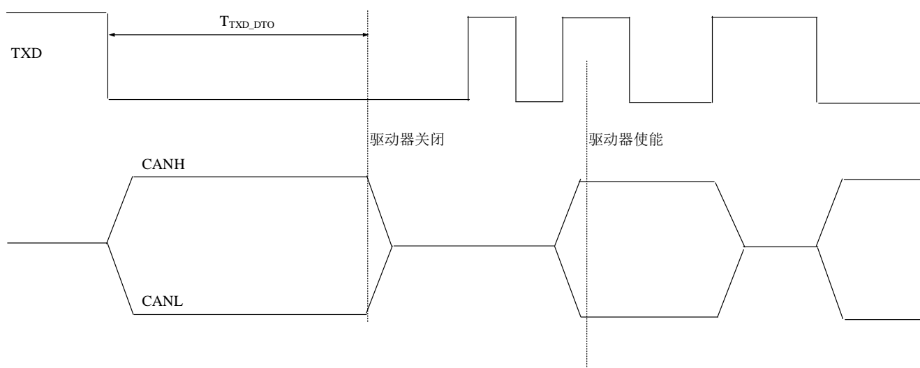
Figure 9-8. Transmitter-Dominant Timeout Protection
