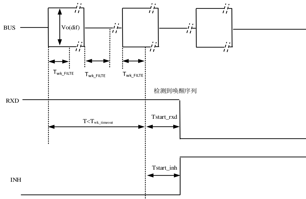
Figure 9-5. Remote Wake-up
