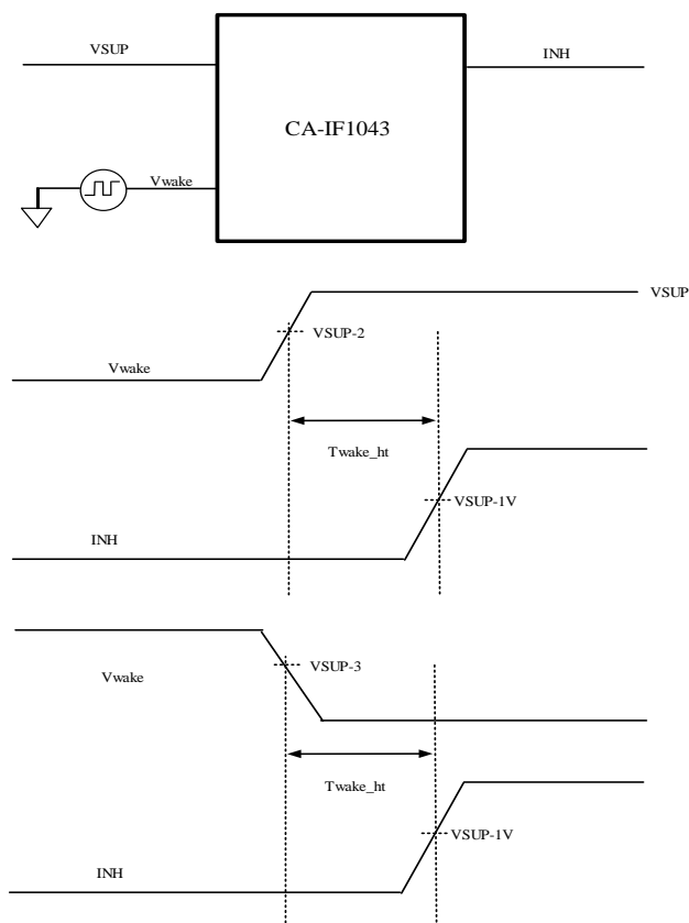
Figure 8-10. INH Response
