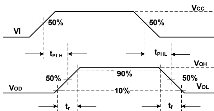
Figure 8-2. Driver Propagation Delays
