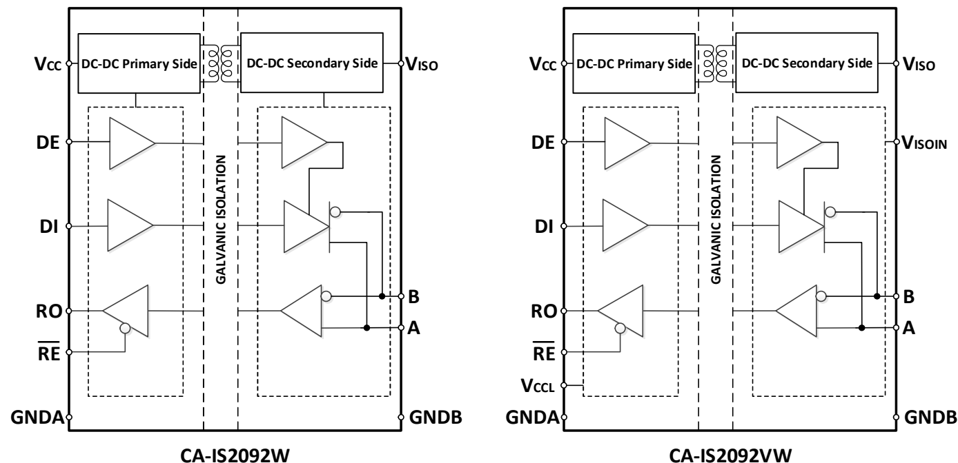
CA-IS2092X Function Diagram
