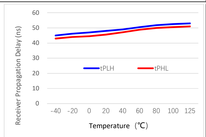
Figure 7-10. CA-IS2092x receiver propagation delay V CC = 3.3V, V ISO = 3.3V, R L = 54Ω
