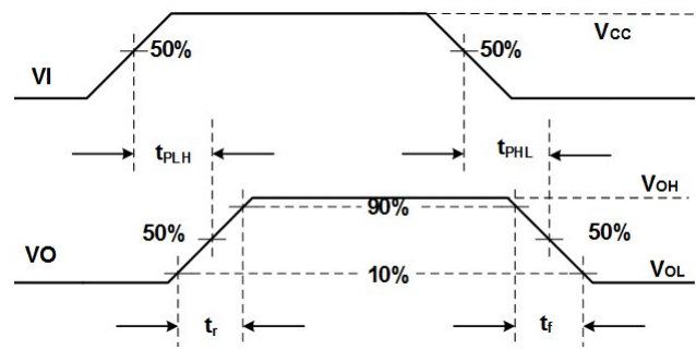
Figure 8-4. Receiver Propagation Delays
