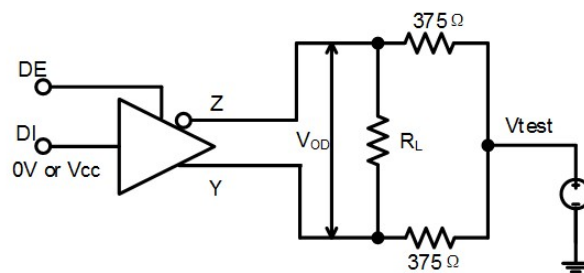
Figure 8-1. Driver DC Test Circuit
