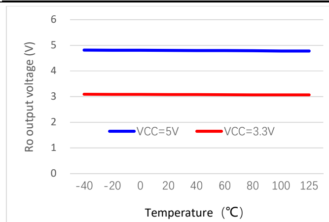
Figure 7-7. Ro = High, Ro pull-down current = 4mA
