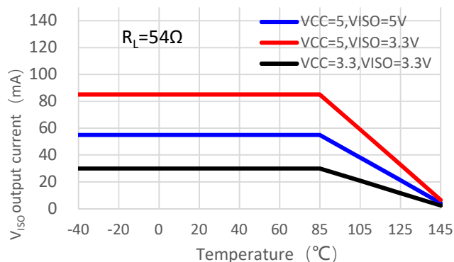
Figure 7-18. Maximum output current from V_{ISO} vs. temperature with R_L = 54\Omega CA-IS2092x: DR = 500kbps, C_L = 2nF
