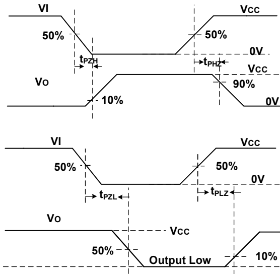
Figure 8-5. Receiver Enable and Disable Times
