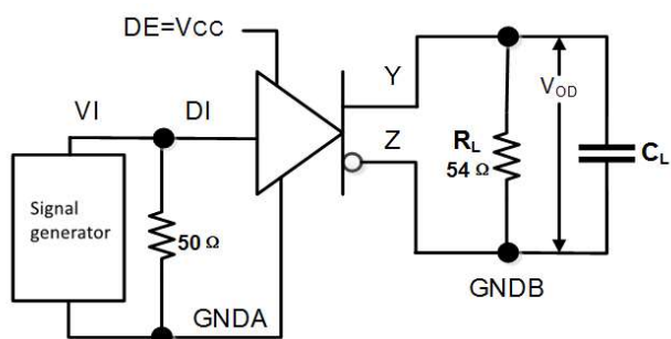
Figure 8-2. Driver Propagation Delays
