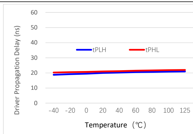
Figure 7-9. CA-IS2092x driver propagation delay V CC = 3.3V, V ISO = 3.3V, R L = 54Ω
