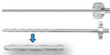
FIGURE 2: THERMOWELLS (TOP: STANDARD, BOTTOM: HELICAL STRAKE TYPE)
