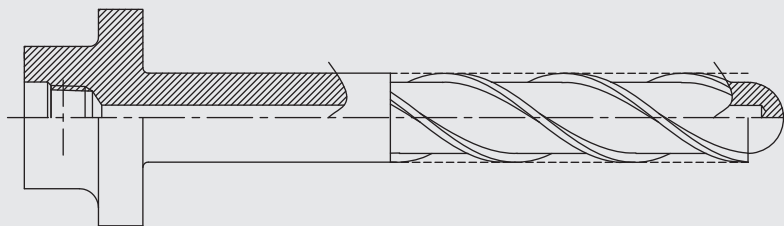
VANSTONE TYPE
