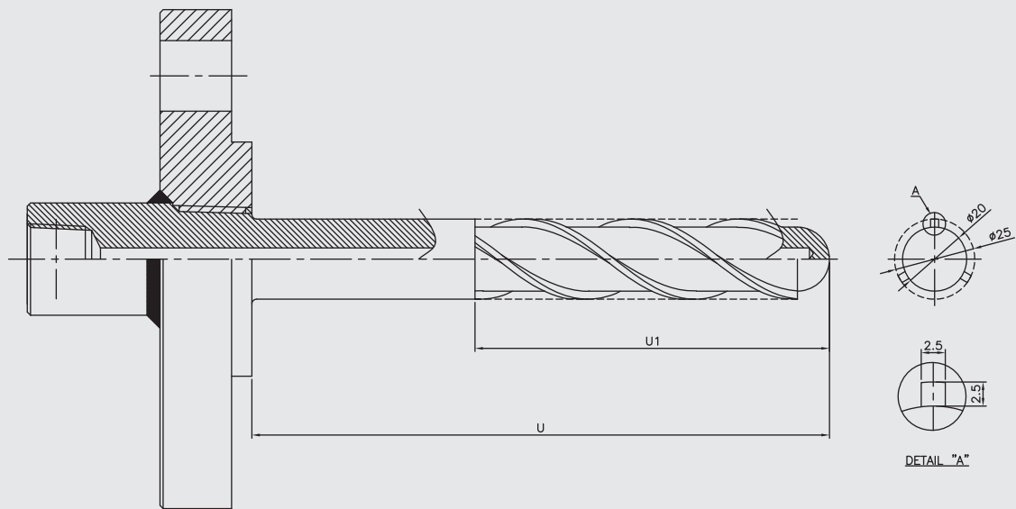
FLANGED TYPE
