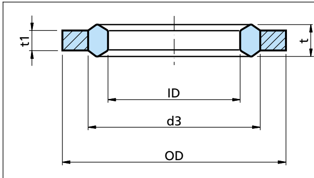
Figure 33 GM1000
