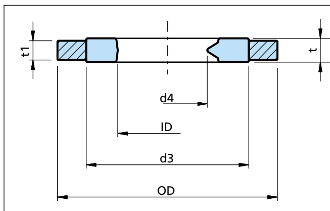
Figure 34 GM2000
