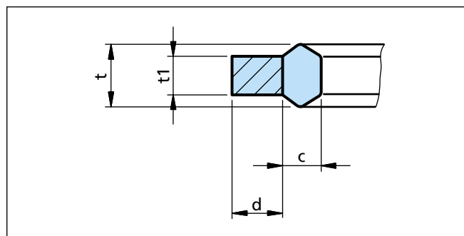
Figure 28 Sealing lip GM3000
