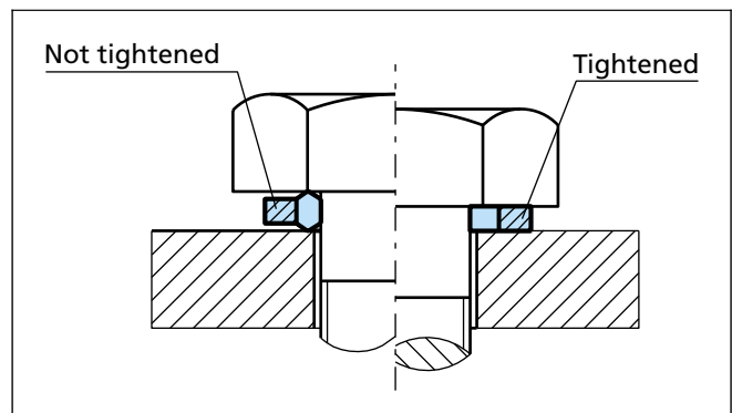
Figure 23 Installation GM1000
