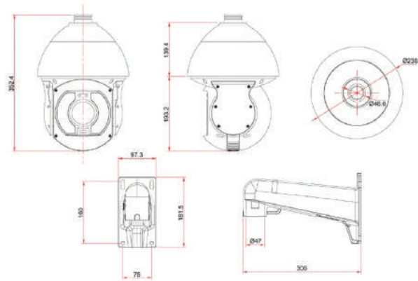
FW8709-QNR 4MP Laser and IR Speed Dome
