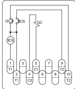
Non-drawout Type
