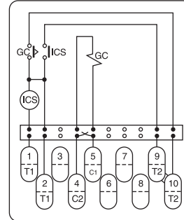
Drawout Type
