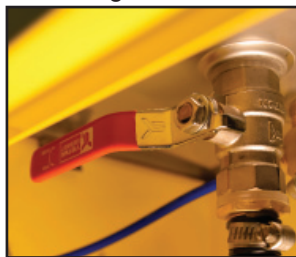
DRAIN VALVE IS OPEN (HANDLE IN VERTICAL POSITION).
