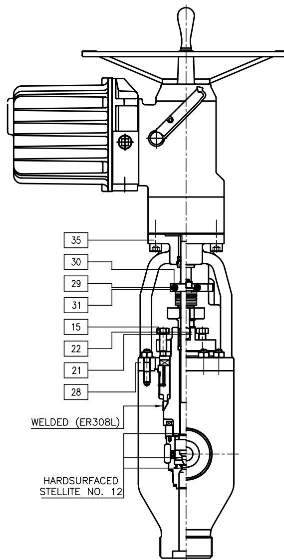
DETAIL OF SEAT & STEM-DISC
