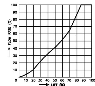
FLOW CHARACTERISTICS CURVE
