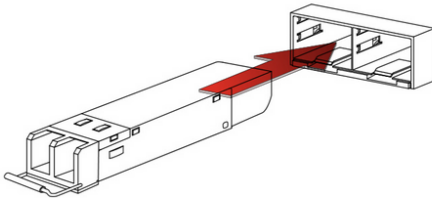
Plug-in the SFP transceiver
