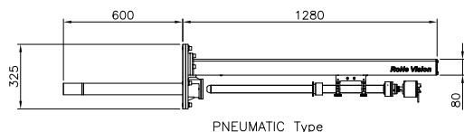
PNEUMATIC Type
