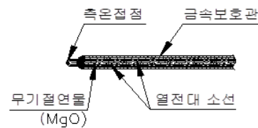
노출형 (Exposed)
