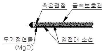
비접지형 (Ungrounded)
