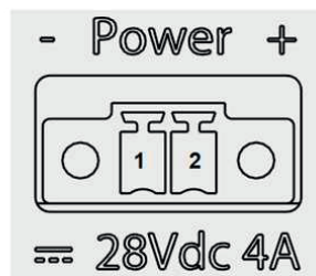
Front view of the receptacle
