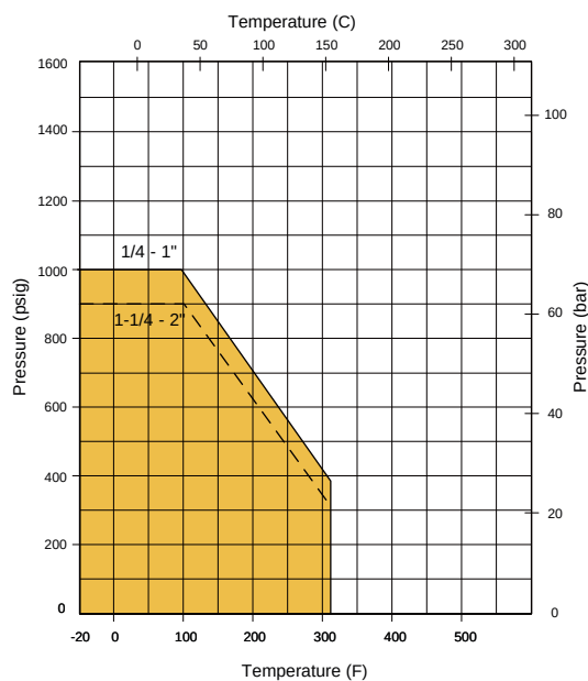
P-TFE Seat and Packing
