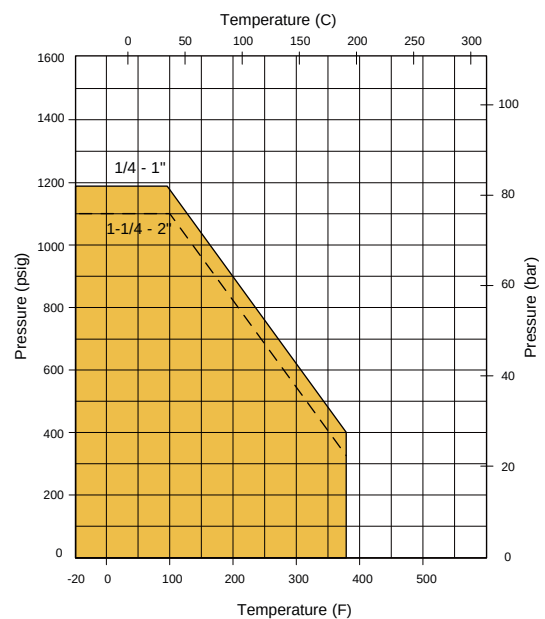
R-TFE Seat and Packing
