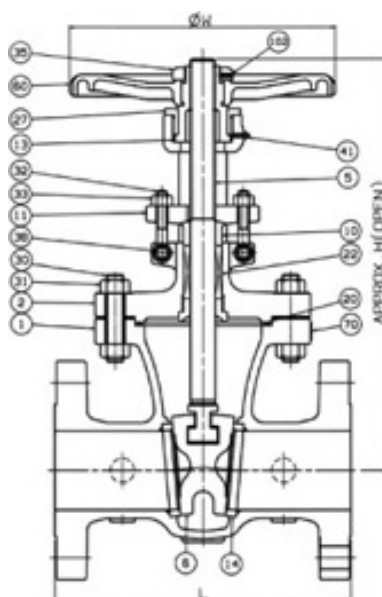
L1(BUTT WELDING) CLASS 300
