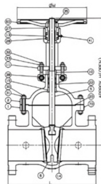
L1(BUTT WELDING) CLASS 600
