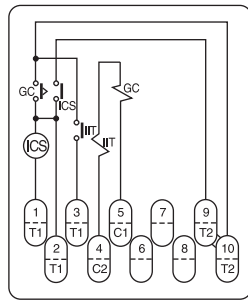
Non-drawout Type
