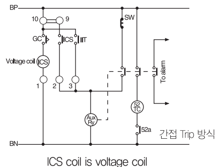
ICS coil is voltage coil
