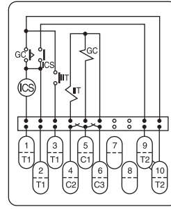
Drawout Type
