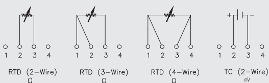
Wiring Diagram
