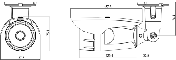
FW7902-PVF 5MP Fixed Bullet
