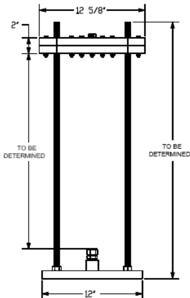
RETRACTOR ASSEMBLY
