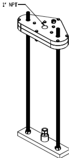
RETRACTOR ASSEMBLY
