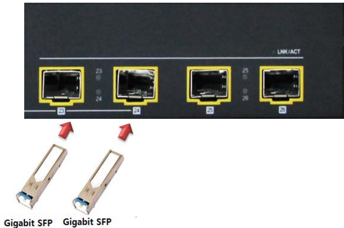
Plug-in the SFP transceiver
