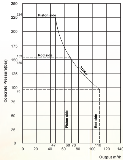
Performance Diagram (ELP15000HP)
