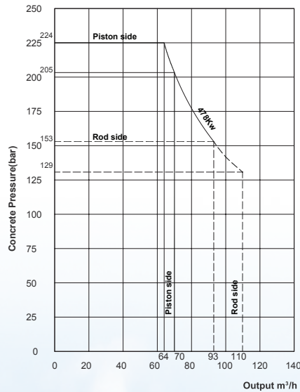
Performance Diagram (ELP1115HP)
