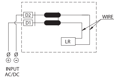
7~12번 (Contact block no. 7 to 12)
