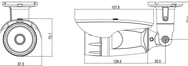
FW7902-FTF 2MP Fixed Bullet
