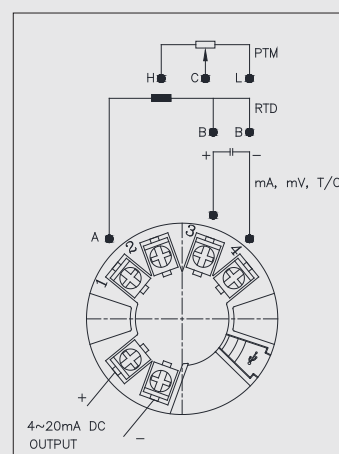
Electrical connection
