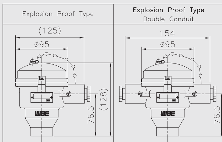
Head
