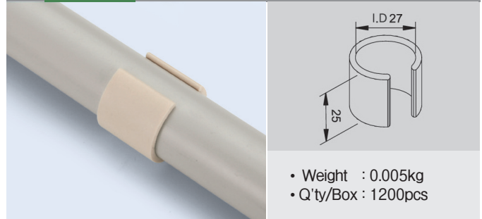
GAP-09-C Grip Bushing (Coating Pipe: Ø28 × T1.0)
