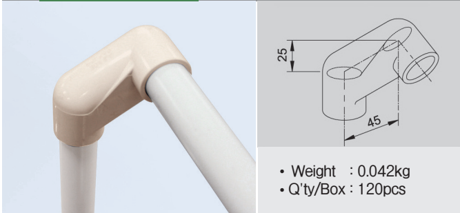
GAP-09-S Grip Bushing (STS Pipe: Ø28 × T0.7)
