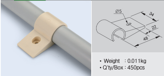
GAP-10L/GAP-10R Plastic Joint
