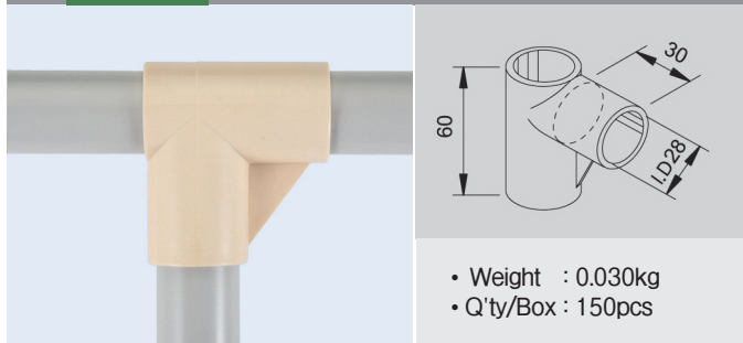
GAP-02A Plastic Joint
