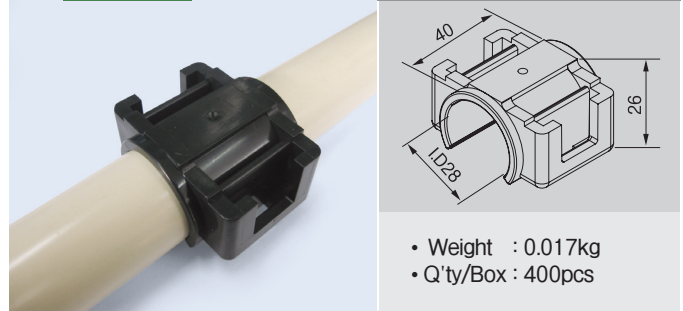
GAP-51 Roller Conveyor Support
