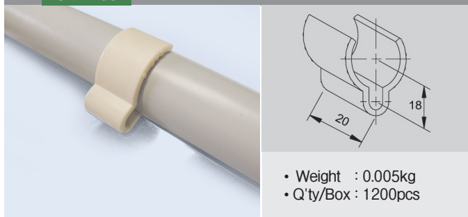
GAP-06 Label Holder
