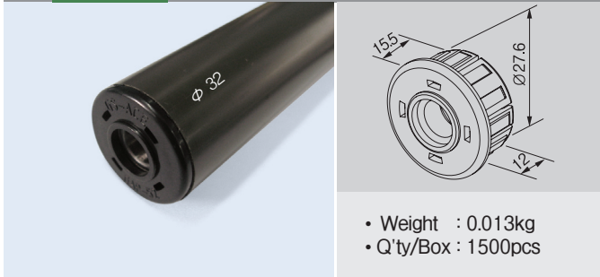
GAP-52A Roller Conveyor Cap (With Bearing)
