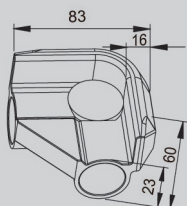
GAP-14 Plastic Joint Corner Cusion Type
