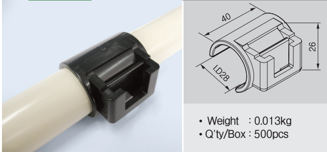
GAP-50 Roller Conveyor Cap (Without Bearing)
