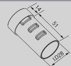
GAP-44 Sleeve (For GA-12S/17S/18S/24S/25S)
