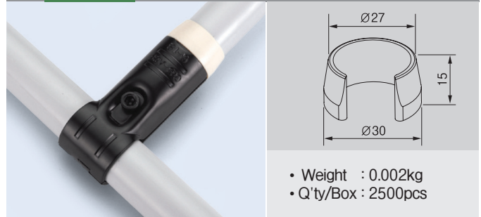
GAP-13 Plastic Joint Corner
