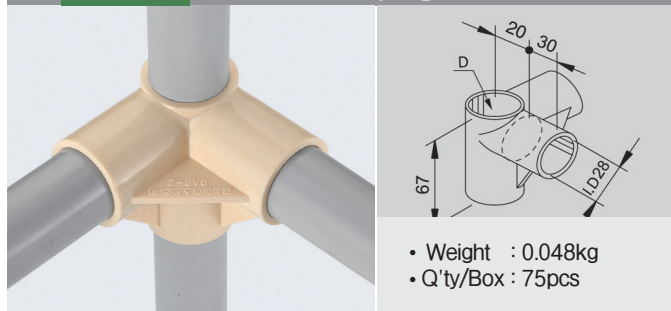
GAP-05 Plastic Joint Corner
