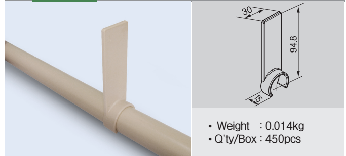
GAP-53 Plastic Joint
